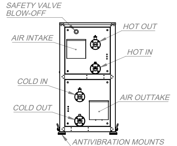
RIGHT VIEW
