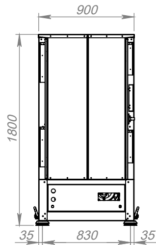
LEFT VIEW
