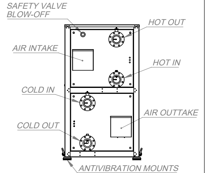
RIGHT VIEW
