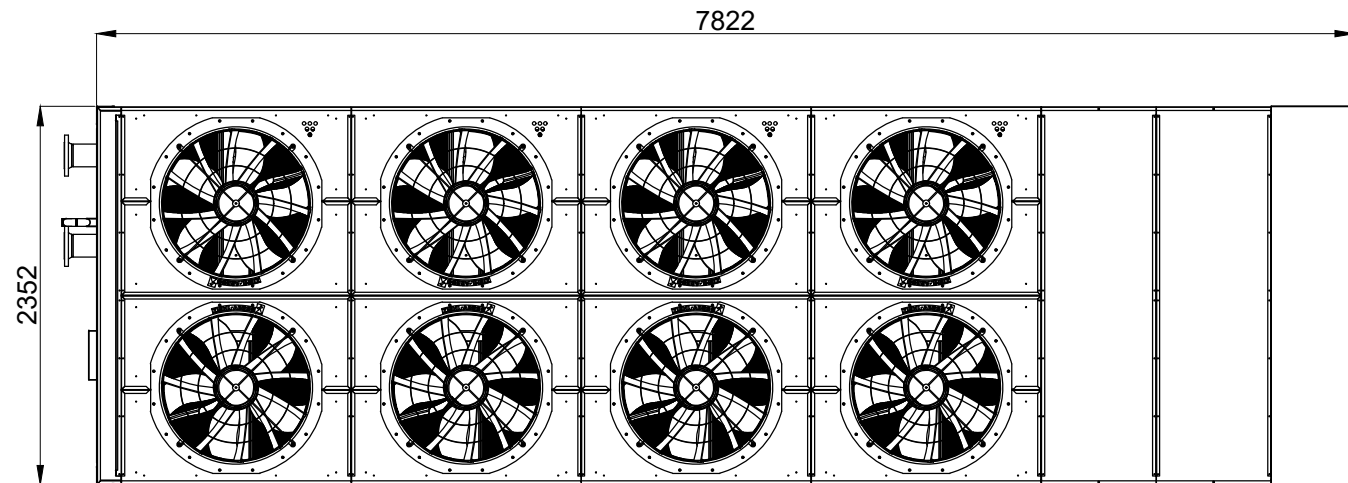
FRONT VIEW
