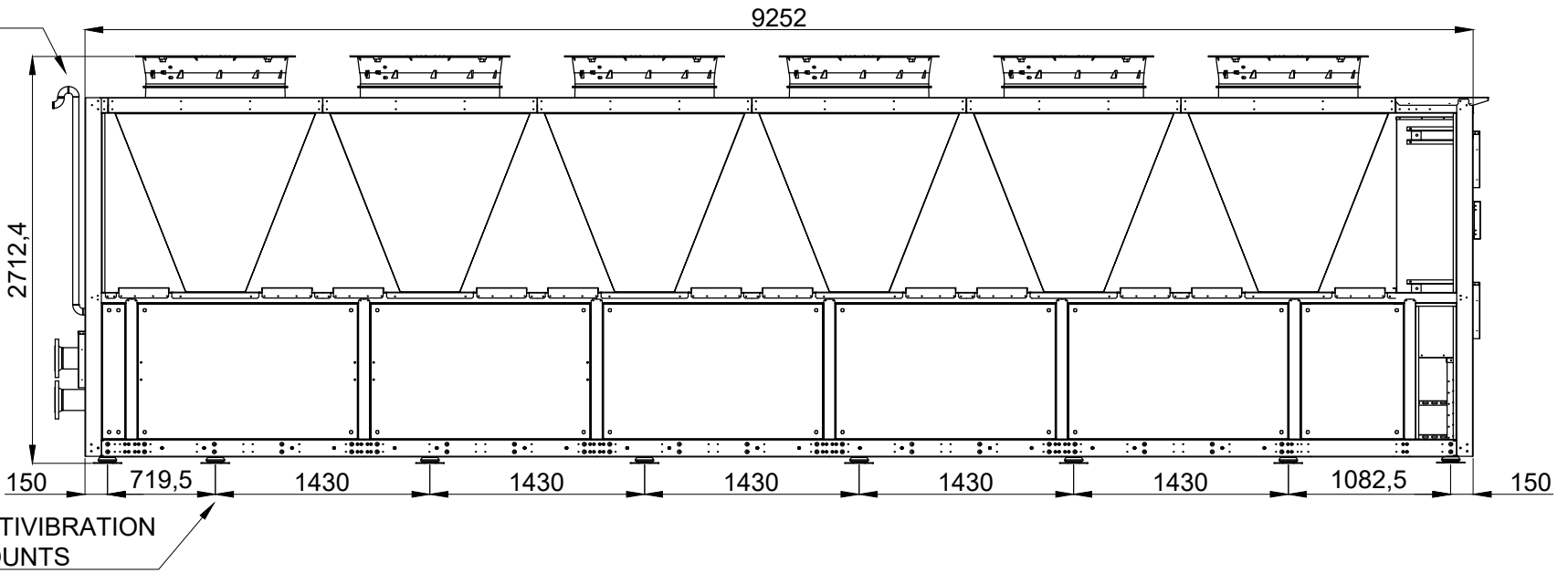
FRONT VIEW
